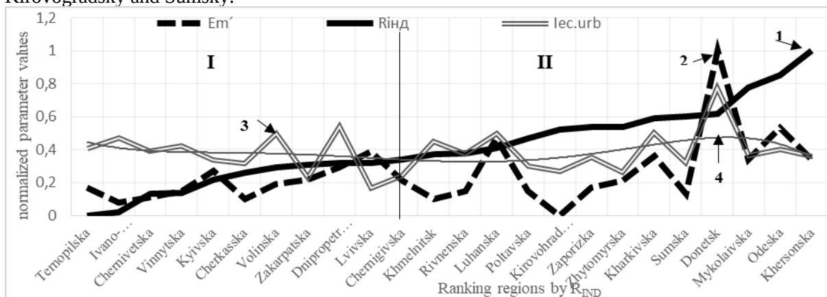
Fig. 1. Coupling between Individual risk levels of the population of Ukraine regions, amount of emergencies (2009 – 2019) and the ecological urbanization index: 1 – R_{ind} ; 2 – E_m' ; 3 – I_{ec.urb} ; 4 – trend line I_{ec.urb}
