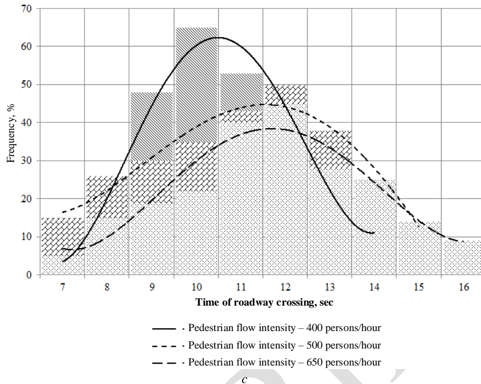
Fig. 3. Distribution of average time which pedestrians spend on crossing the roadway: a – suburban zone (zone near suburban railway station), roadway width 28 m; b – central zone, roadway width 18 m; c – residential zone, roadway width 18 m
