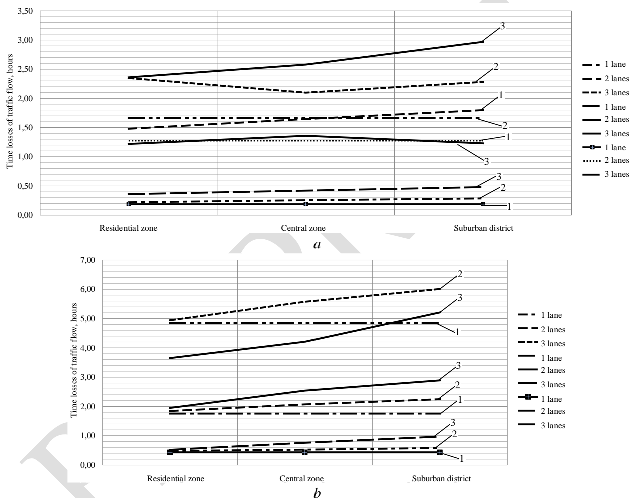
Fig. 5. Distribution of time losses of traffic flows during an hour on intersections which are located in different functional zones of the city: a – at one-way movement; b) – at two-way movement; 1 – by the method of Klinkovshteyn without considering pedestrian behavior; 2 – by the method of Klinkovshteyn with considering pedestrian behavior; 3 – based on program software VISSIM
