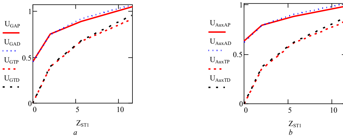
Fig. 3 Voltage dependence for digital (D) and physical (P) scheme models of the PU with an AAT(A) and a traditional scheme of the PU without an AAT (T) from resistance Z_{ST1} : a - U_G^* ; b - U_{Aux}^* .
