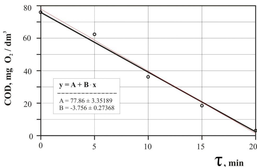
Fig. 4. Dependence of the COD change of sewage on the time of electrical treatment at the first stage of influence
