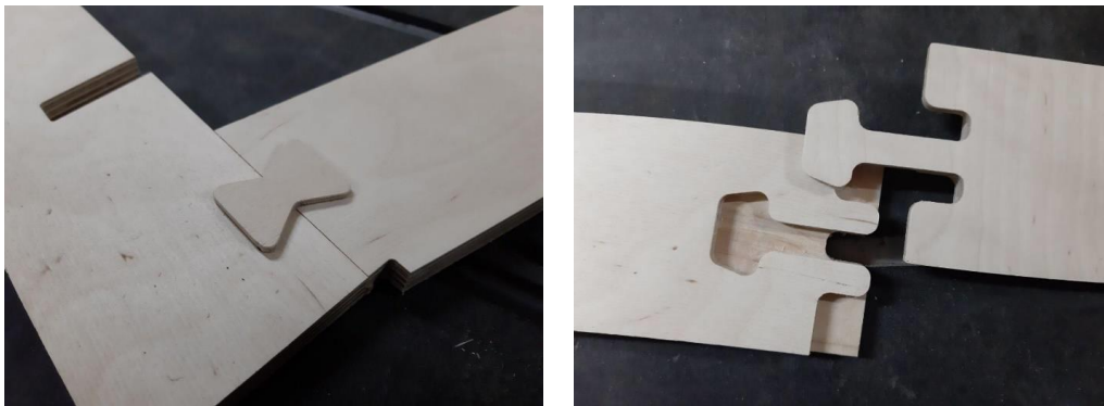
Fig. 1 a, b. Technological nodal joints are made on a CNC machine
