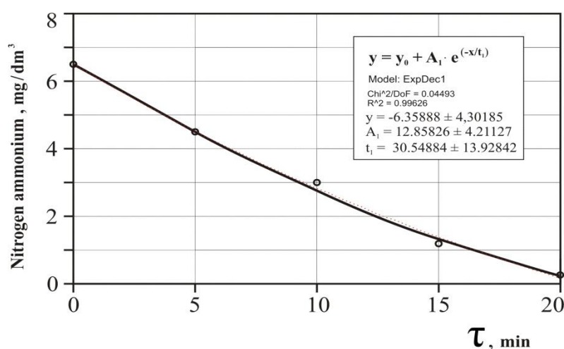
Fig. 5. Change in the amount of ammonium nitrogen depending on the filtration time in the second stage
