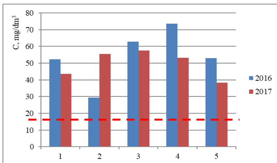
Fig. 4. Change of the suspended matter content in the surface waters of Lviv in 2016-2017 (1 – the Lysynitskyi Stream, 2 – the Kryvchytskyi Stream, 3 – the Bilohorskyi Stream, 4 – Marunka River, 5 – the Kleparivskyi Stream)
