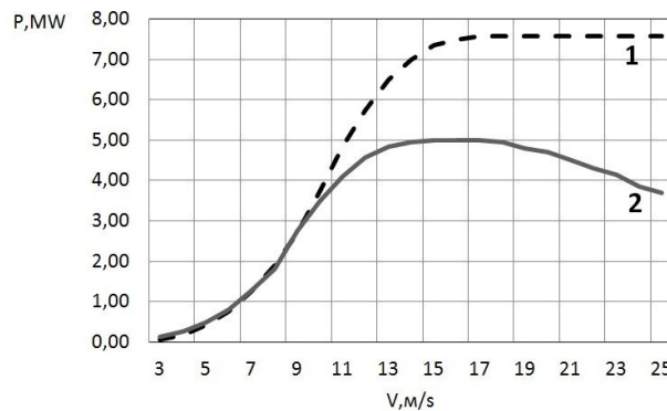
Fig.2. Performance characteristics: 1- Enercon E-126, 2- Gamesa G132.
