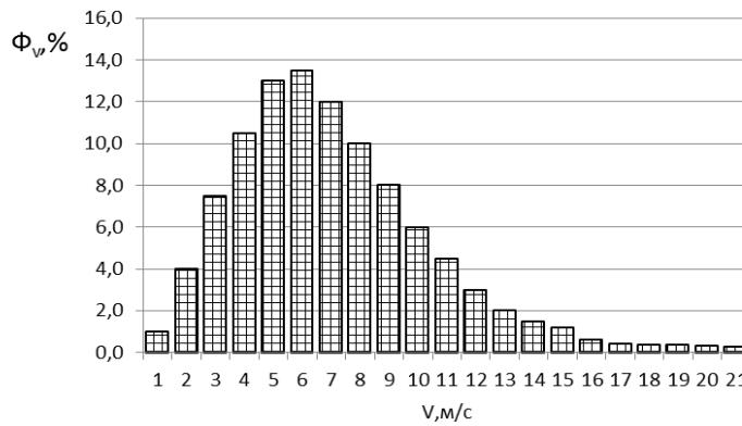
Fig.1. Analytical Weibull distribution.
