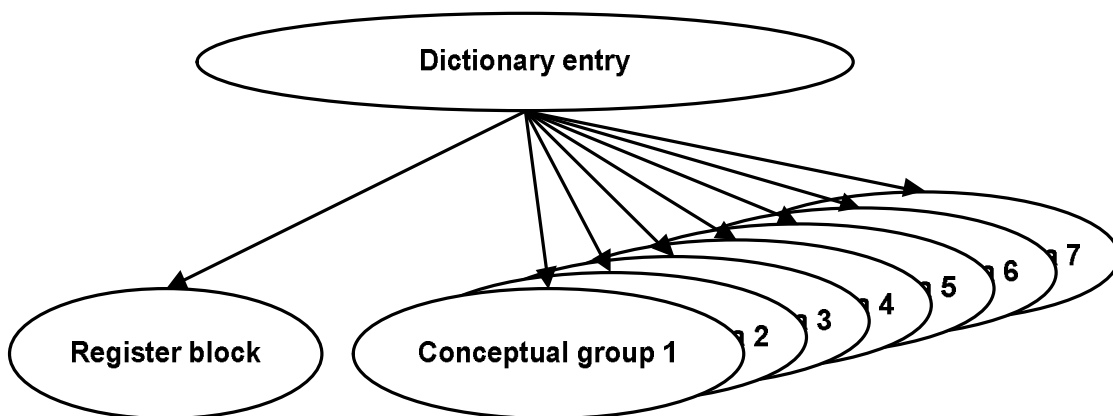
Fig. 3. The generalized structure of the entry of five language dictionary
