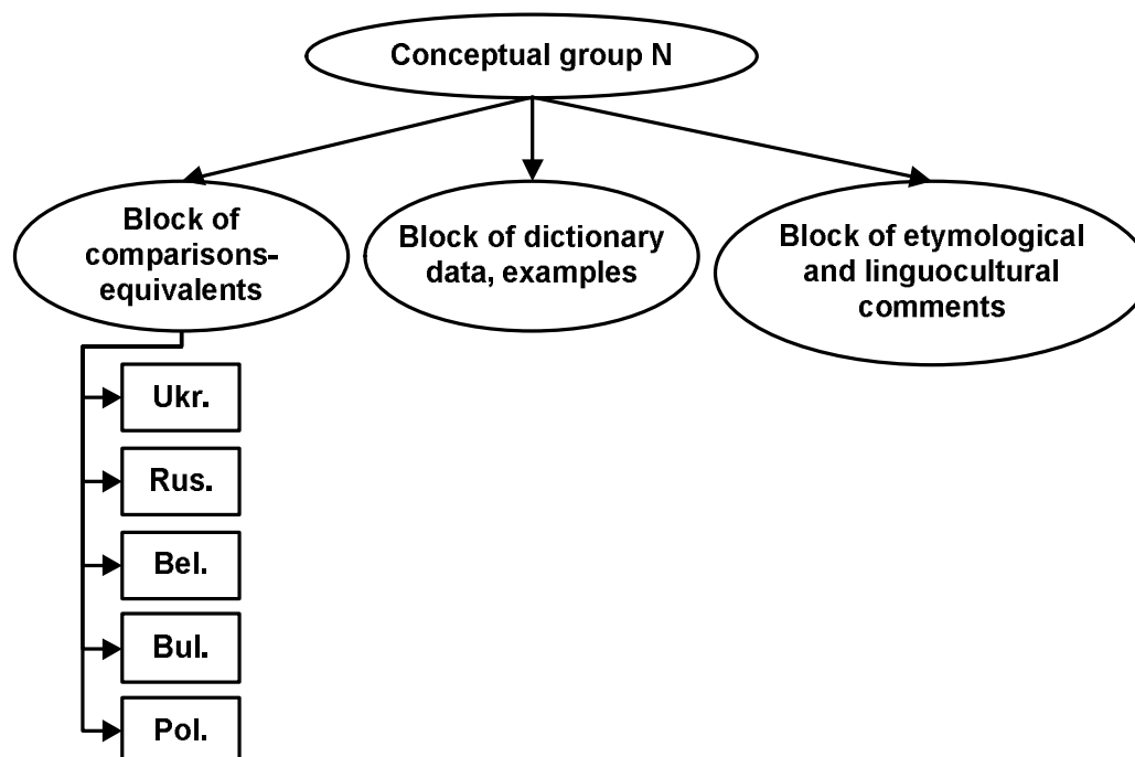
Fig. 5. The structure of the conceptual group of the entry of five language dictionary of comparisons
