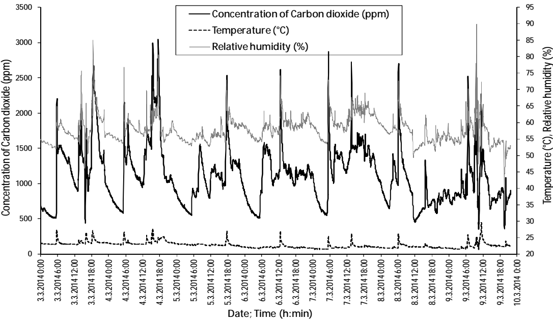
Fig. 2. Variation of indoor air parameters in kitchen
