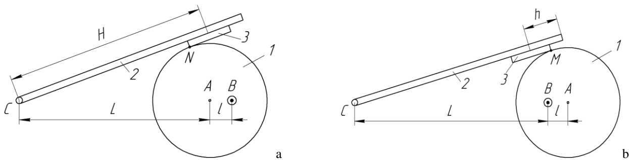
Fig.2. Scheme position a workpiece at various stages of rotation cycloidal special working tools:
