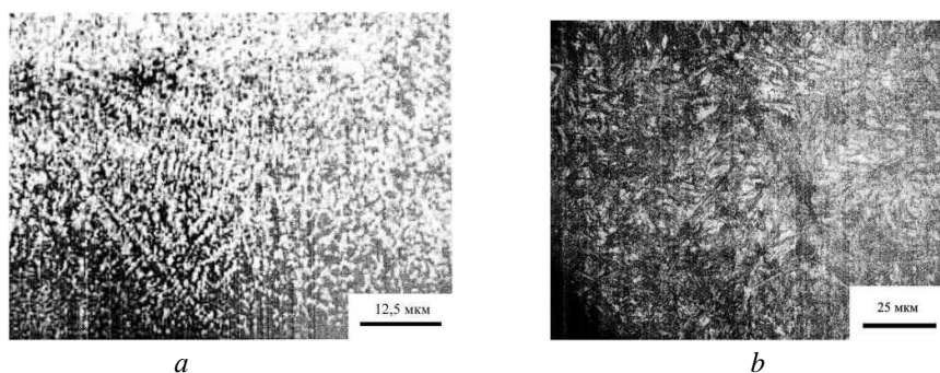
Fig. 1. Microstructure of alloy steel: a) dendritic b) martensite with hardness HRC 63
