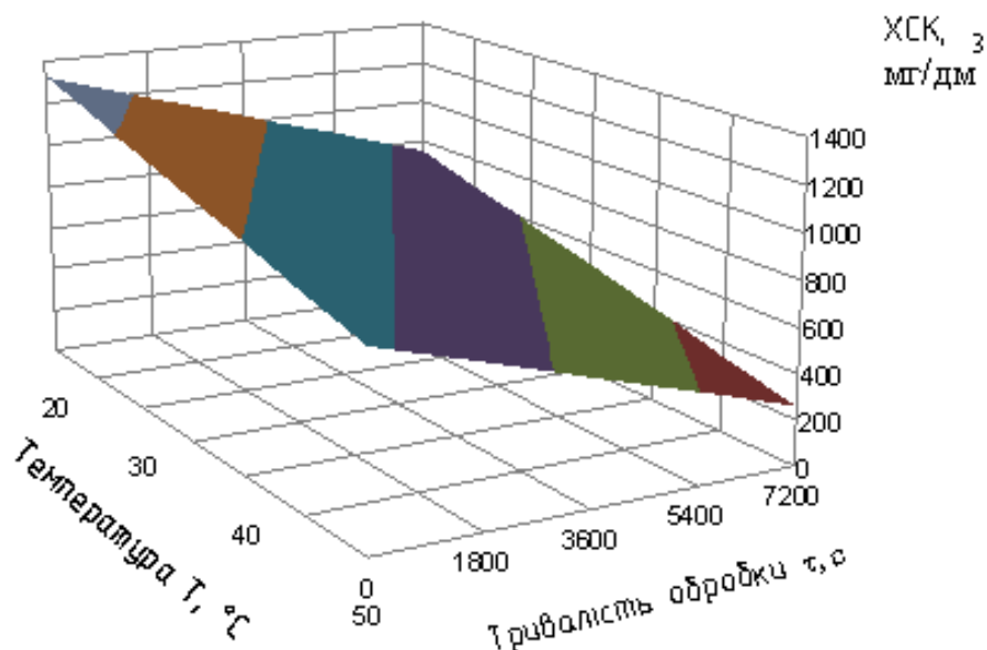
Fig. 2. Graphic reflection of influencing of technological parameters on the indexes of quality of the vibrocavital cleaning of wastewater of «Kumpel» brewing production from organic contaminations
