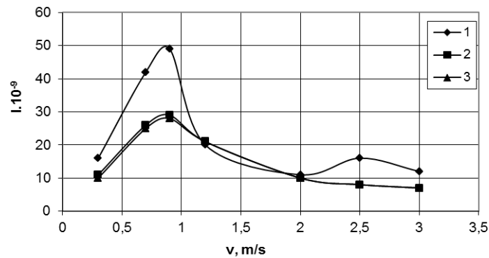
Figure 1. Dependence of wear resistens pair Steel 40X - Steel 40X after frictional hardening tool with different working part of the wear velocity ( P = 1 MPa): 1 - initial, 2 - with a smooth surface, 3 - with the cut slots inclined in different direction.
