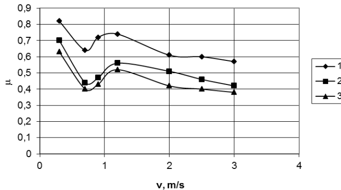
Figure 3. Dependence of friction wear pair Steel 40X - Steel 40X after frictional hardening tool with different working part of the wear velocity ( P = 1 MPa): 1 - initial, 2 - with a smooth surface, 3 - with the cut slots inclined in different direction.
