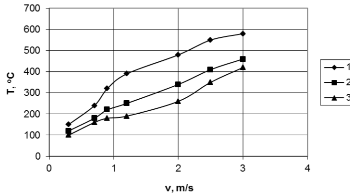
Figure 2. The dependence of the temperature in the contact zone with wear pair Steel 40X - Steel 40X after frictional hardening tool with different working part of the wear velocity ( P = 1 MPa): 1 - initial, 2 - with a smooth surface, 3 - with the cut slots inclined in different direction.
