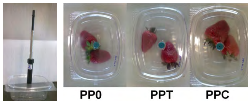
Fig. 1. Experimental assembly used for headspace analysis of whole strawberries by HS-SPME
