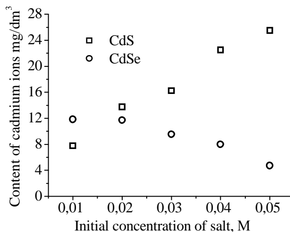
Fig. 1. Dependence of \text{Cd}^{2+} ions content on \text{CdCl}_2 concentration at CSD of CdS and CdSe films. C(\text{CS}(\text{NH}_2)_2) = 1 \text{ M} ; C(\text{Na}_2\text{SeSO}_3) = 0.1 \text{ M} ; T = 343 \text{ K} ; the deposition time is 4 \times 3 \text{ min} .
