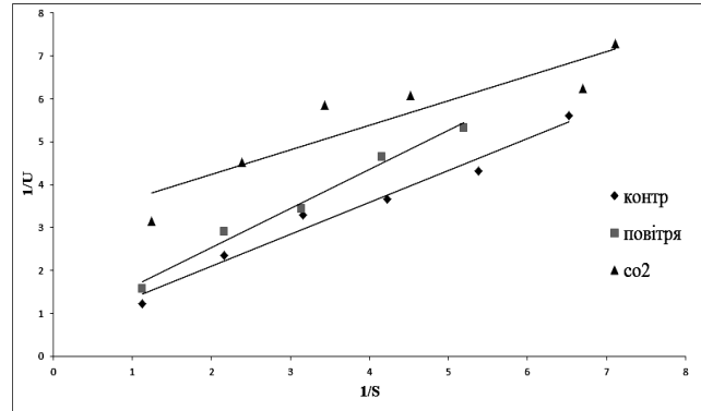
Fig. 7. Dependence of inverse rate growth on substrate concentration
