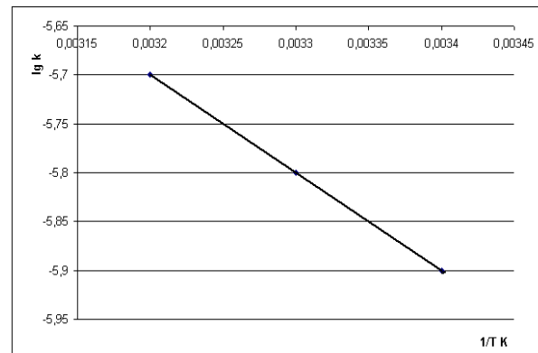
Fig. 4. Logarithm of growth factor k_m vs. 1/T
