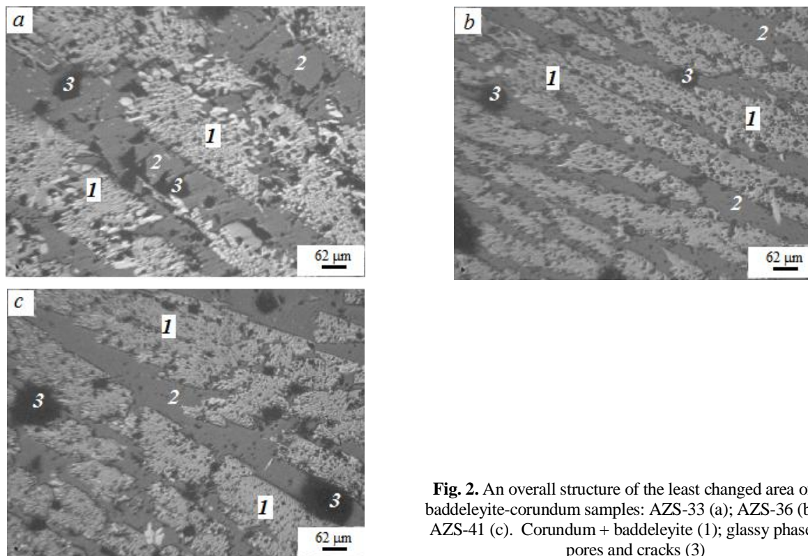
Structure characteristic of the baddeleyite-corundum samples of the least changed area
