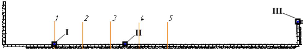
Fig. 1. Scheme of sampling of melting tank lining: axes of the burner portals (1-5); sampling locations (I, II, III)
