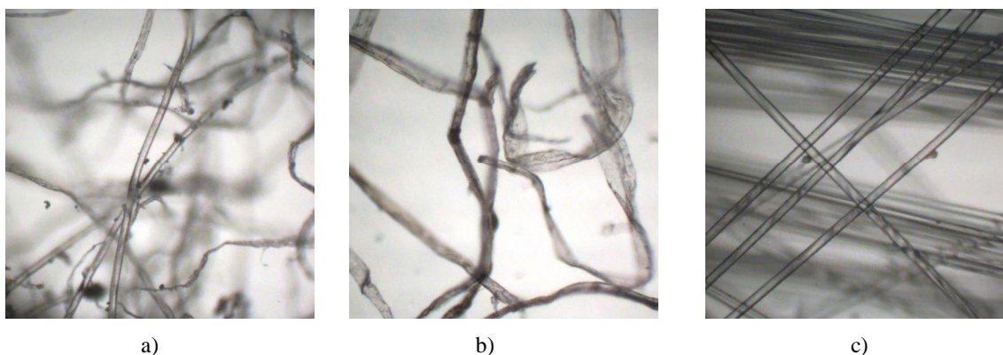
Fig. 3. Microphotographs cellulose fiber obtained during the grinding wastes wall (a), natural fiber paper (b) and PVA fiber used in "Ivano-Frankivsk" (c) to get asbestos cement roofing slate. The sizes of cellulose fibers were: L = 0.1-1 mm; D = 0.01-0.1 mm. Photos were taken with RV-3320 microscope (image scale 1:100)
