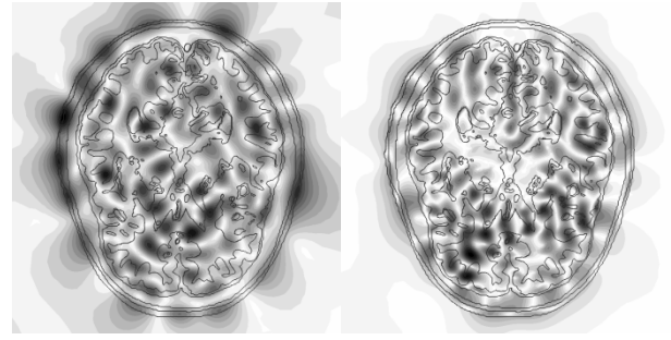
Fig. 7. Example of numerical computation of eigenfrequencies in the human head phantom at 1,775 GHz; left: electric field E , right: magnetic field H . Q_{\text{fact}} = 3,4 .
