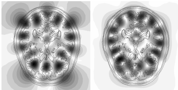
Fig. 6. Example of numerical computation of eigenfrequencies in the human head phantom at 905 MHz; left: electric field E , right: magnetic field H . Q_{\text{fact}} = 2,6 .
