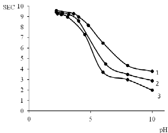
Fig. 1. The dependence of hydroxides SEC (mg \text{Mo/g} ) on pH solution. The initial concentration of molybdenum is 96 mg/l. CPH of the Mn:Fe composition: 3:1 (1); 1:1 (2) and 1:3 (3)
