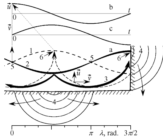
Fig. 2. Oscillations of the standing wave and the deformation field of the reservoir bed:
