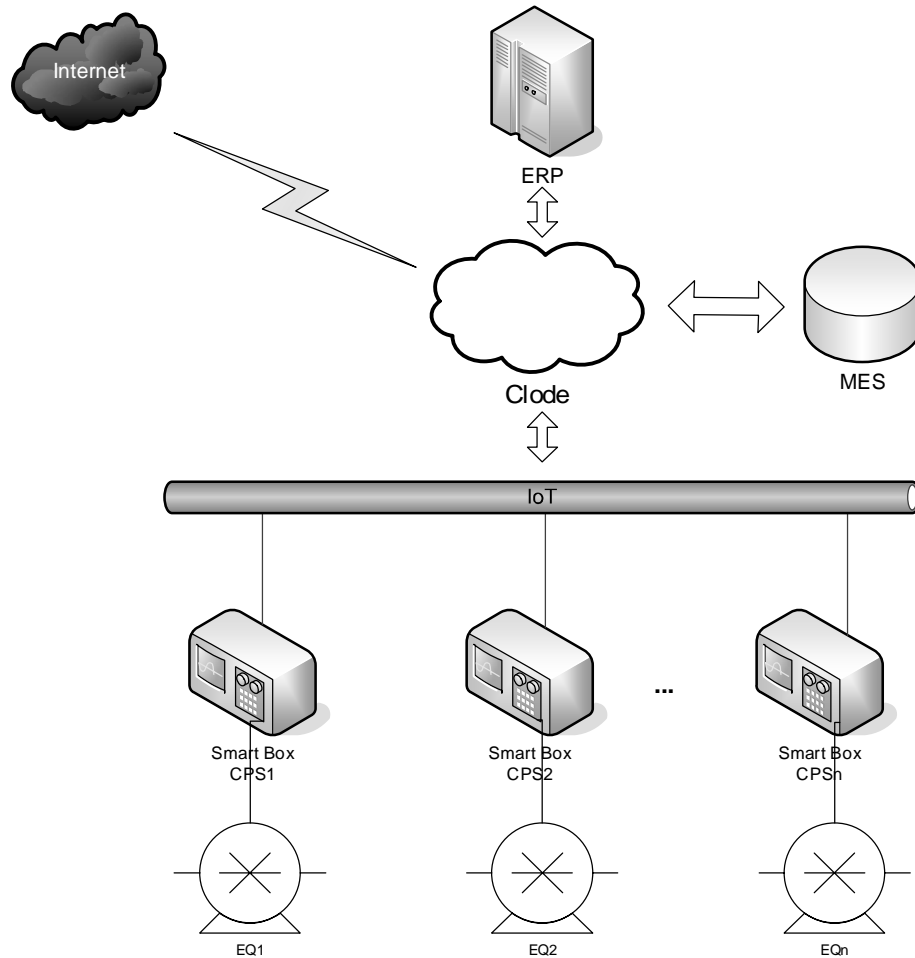
Fig. 4. Intelligence, interconnection
