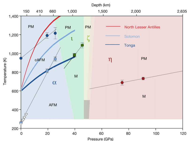
Fig. 3. Magnetic phase diagram of \text{Fe}_2\text{O}_3
