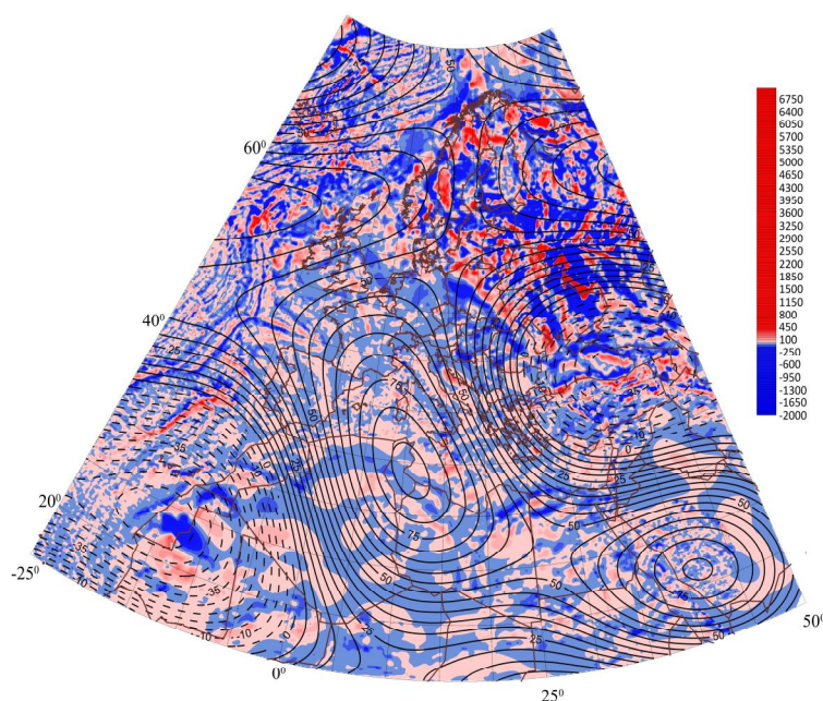
Fig. 1. Scheme of comparison of the Central European crustal-mantle anomaly (isolines, nT) by [Orlyuk, et al., 2019] with anomalous magnetic field (WDMAM) by [Dyment, et al., 2016] Brown lines – contours of coastlines
