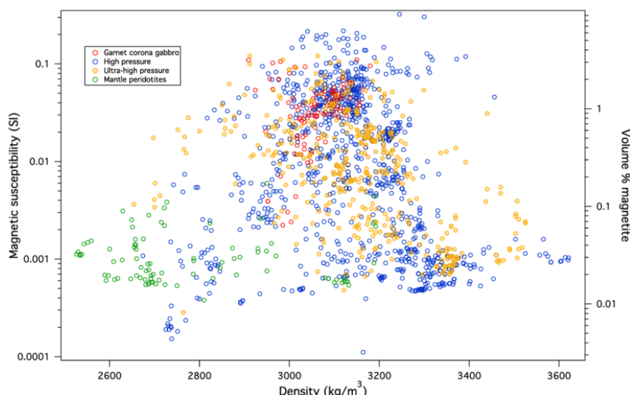
Fig. 2. Magnetic susceptibility (left axis) and estimated magnetite content (right axis) as function of density [McEnroe, et al., 2018]
