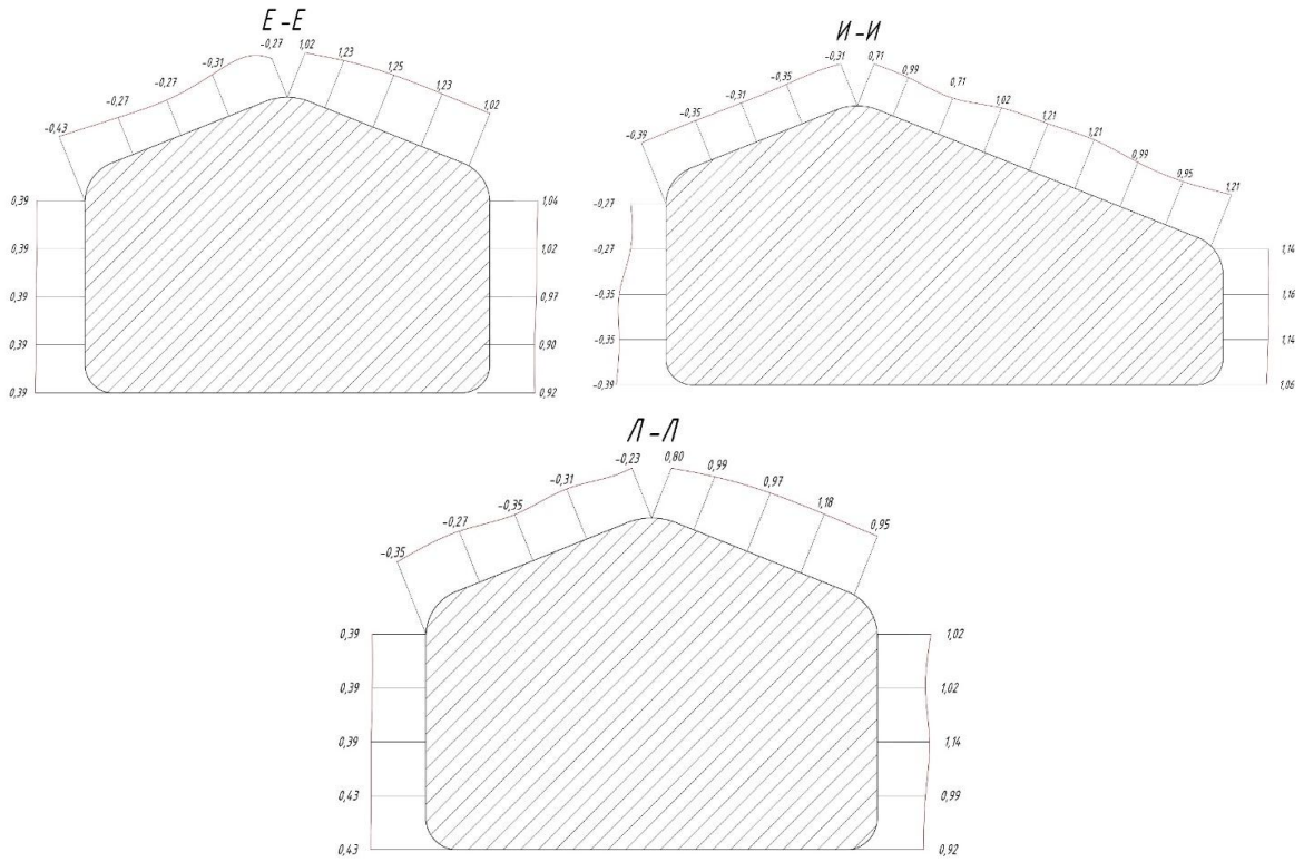
Fig. 5. Plots of the distribution of aerodynamic coefficients in section E-E, И-И, Л-Л for the direction of the incoming wind stream \alpha = 0^\circ .
