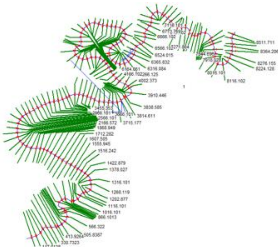
Fig. 8. Data visualization for modeling using HEC-RAS software
