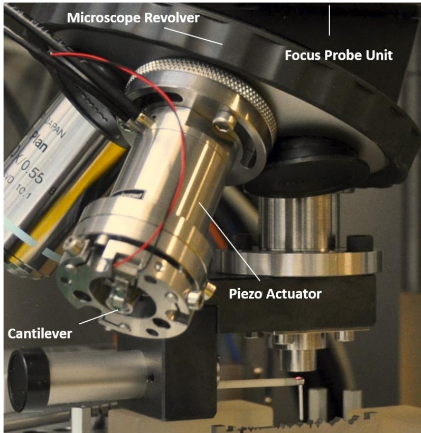
Figure 7. Atomic force sensor in the NPM Machine.
