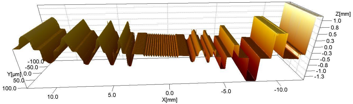
Figure 9. Microcountour measured with the DFF method.
