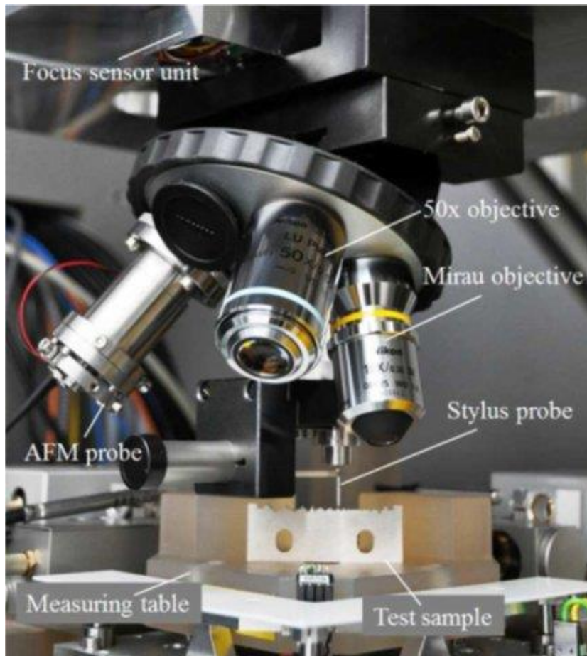
Figure 10. Microscope revolver approach.
