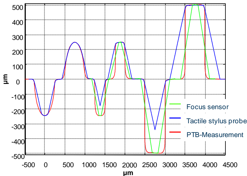
Figure 8. Comparison of micro contour measurements.
