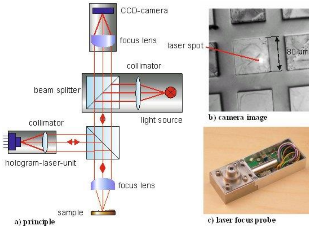
Figure 3. Laser focus probe.
