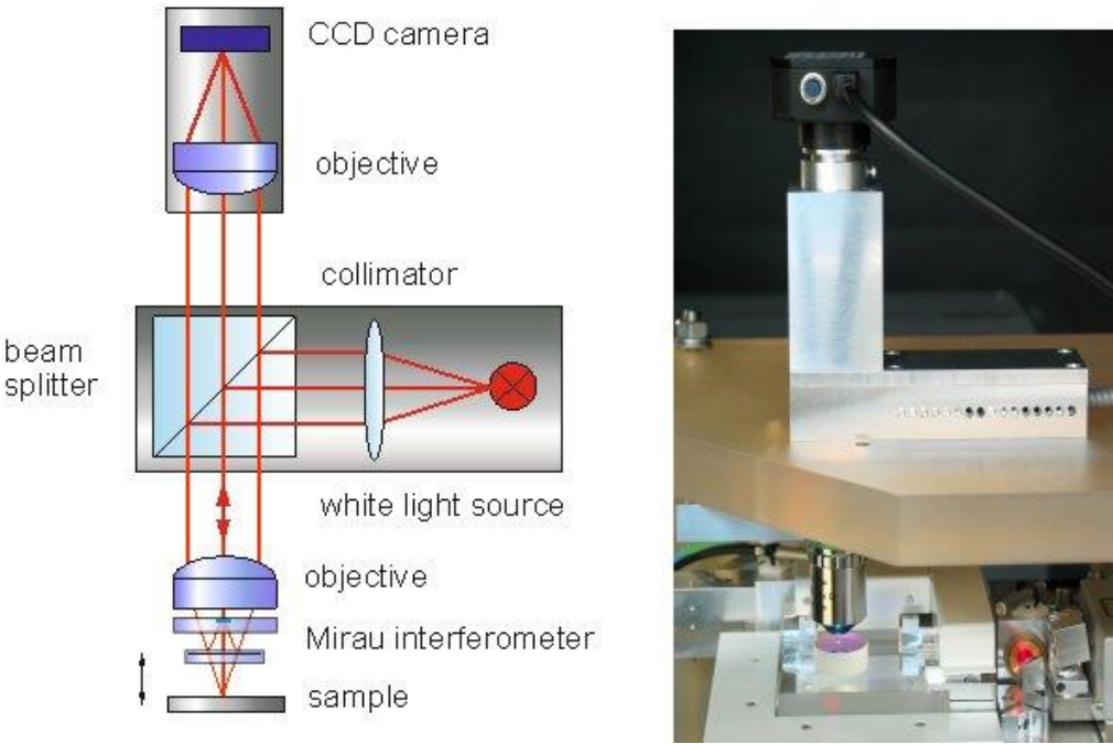
Figure 5. White-light interference microscope.
