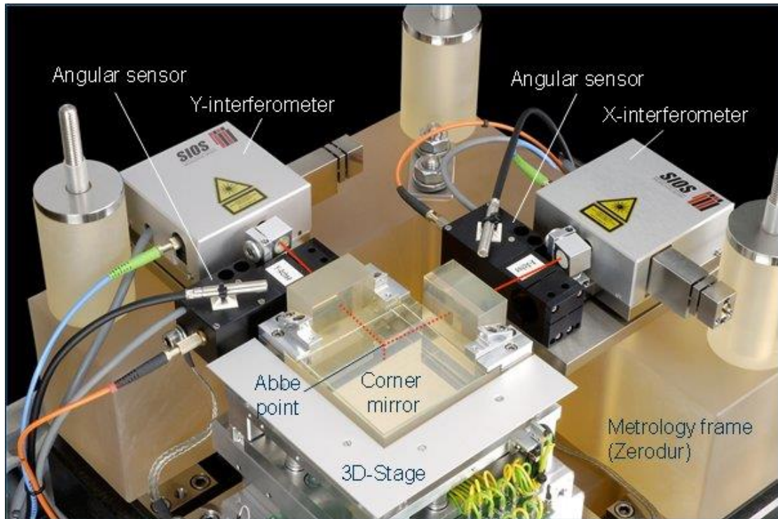
Figure 2. Basic components of the NMM-1.
