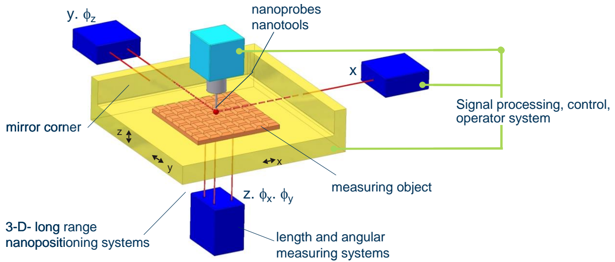
Figure 1. The basic concept and main components of the NPM-machine.
