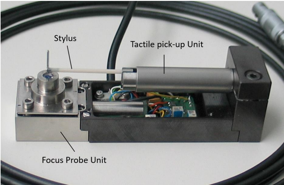
Figure 6. Tactile stylus probe.
