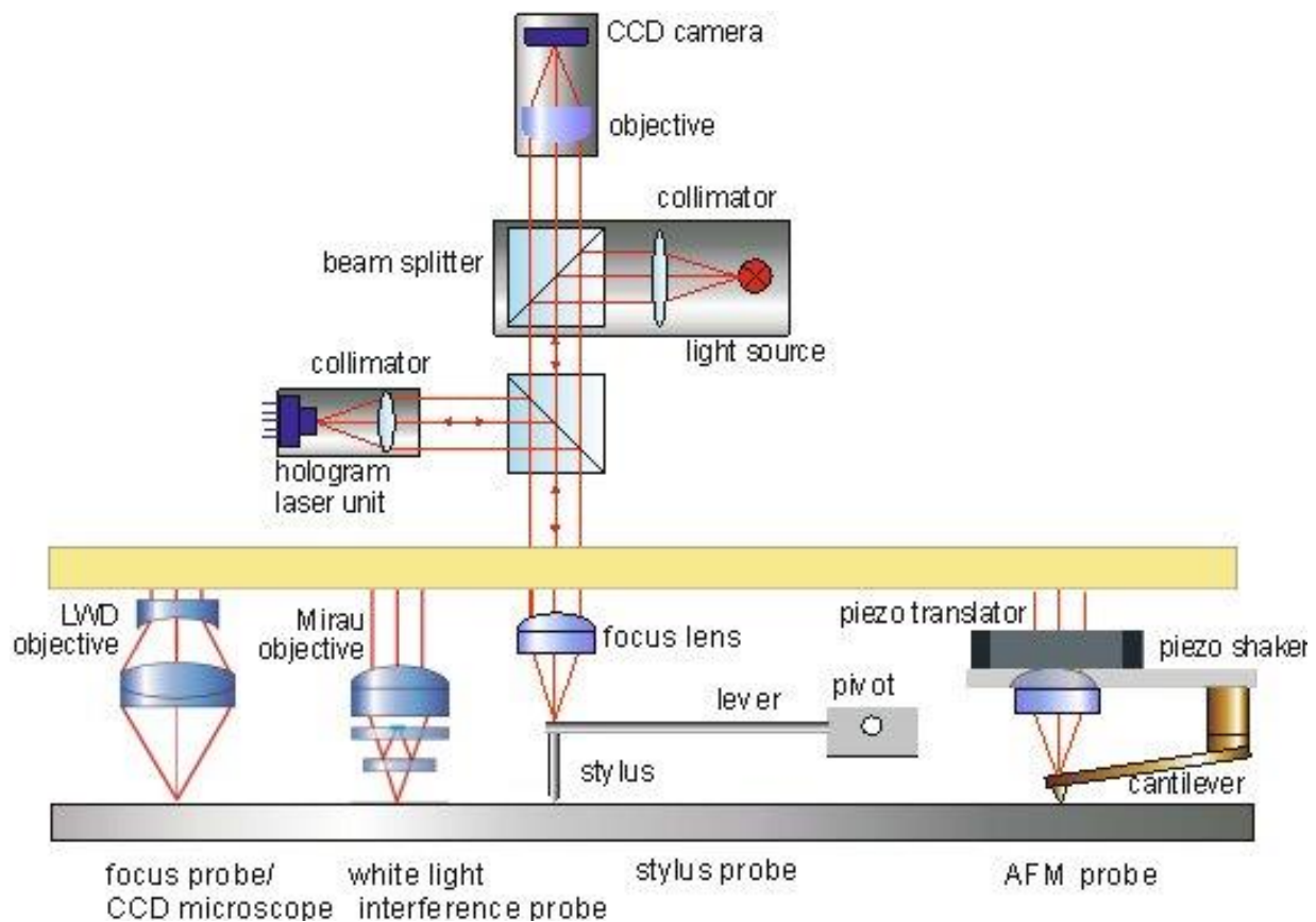
Figure 4. Several probing systems based on laser focus probe.
