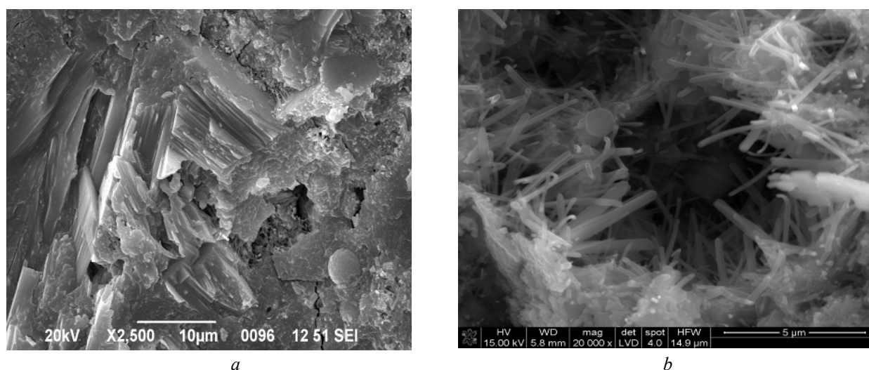
Fig. 1. Microstructure of superplasticized cement stone after 28 days: crystals of portlandite ( a ) and dispersible crystals of ettringite ( b )
