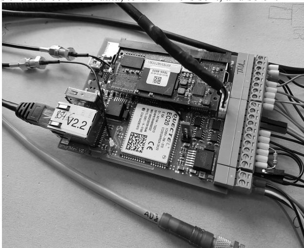
Fig. 7. Data transmitter and encoder
