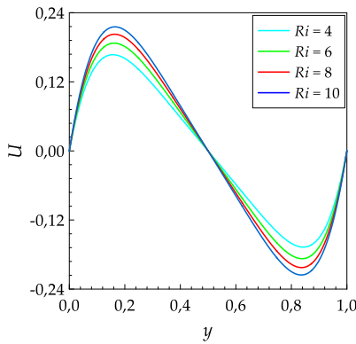
Fig. 4. Longitudinal velocity profiles along the mid-plane x = 0.5 for various values of Ri , when \chi = 0.01 and d_{np} = 30 nm.
