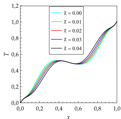
Fig. 8. Horizontal temperature profiles along the mid-plane y = 0.5 for various values of \chi , when Ri = 8 and d_{np} = 30 nm.
