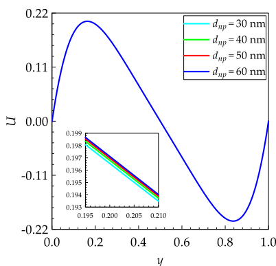
Fig. 10. Longitudinal velocity profiles along the mid-plane x = 0.5 for various values of d_{np} , when Ri = 8 and \chi = 0.01 .
