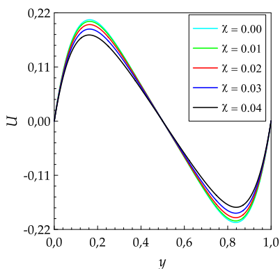
Fig. 7. Longitudinal velocity profiles along the mid-plane x = 0.5 for various values of \chi , when Ri = 8 and d_{np} = 30 nm.
