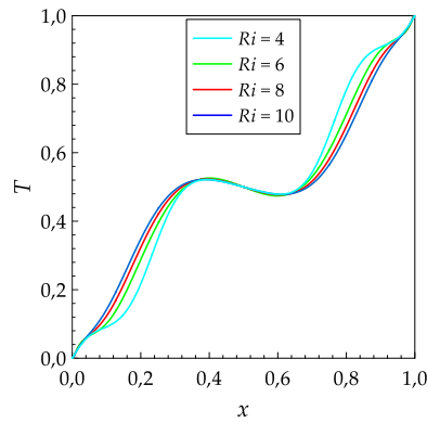
Fig. 5. Horizontal temperature profiles along the mid-plane y = 0.5 for various values of Ri , when \chi = 0.01 and d_{np} = 30 nm.
