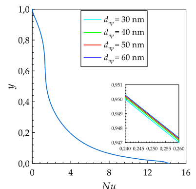
Fig. 12. Local Nusselt number profiles at the vertical cold wall x = 0 for various values of d_{np} , when Ri = 8 and \chi = 0.01 .
