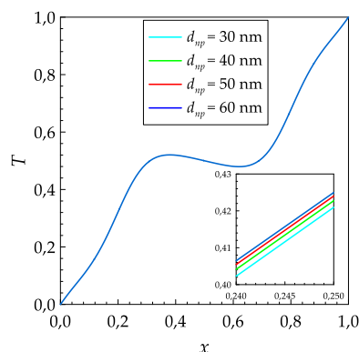
Fig. 11. Horizontal temperature profiles along the mid-plane x = 0.5 for various values of d_{np} , when Ri = 8 and \chi = 0.01 .
