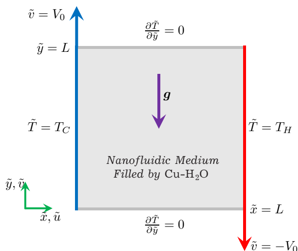
Fig. 1. Geometrical configuration of the present convective nanofluid flow problem.
