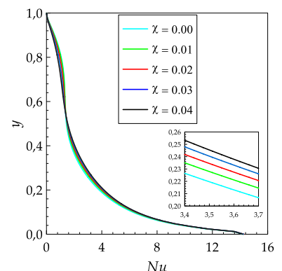
Fig. 9. Local Nusselt number profiles at the vertical cold wall x = 0 for various values of \chi , when Ri = 8 and d_{np} = 30 nm.
