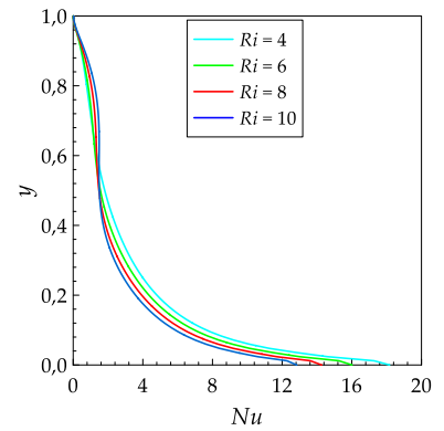
Fig. 6. Local Nusselt number profiles at the vertical cold wall x = 0 for various values of Ri , when \chi = 0.01 and d_{np} = 30 nm.
