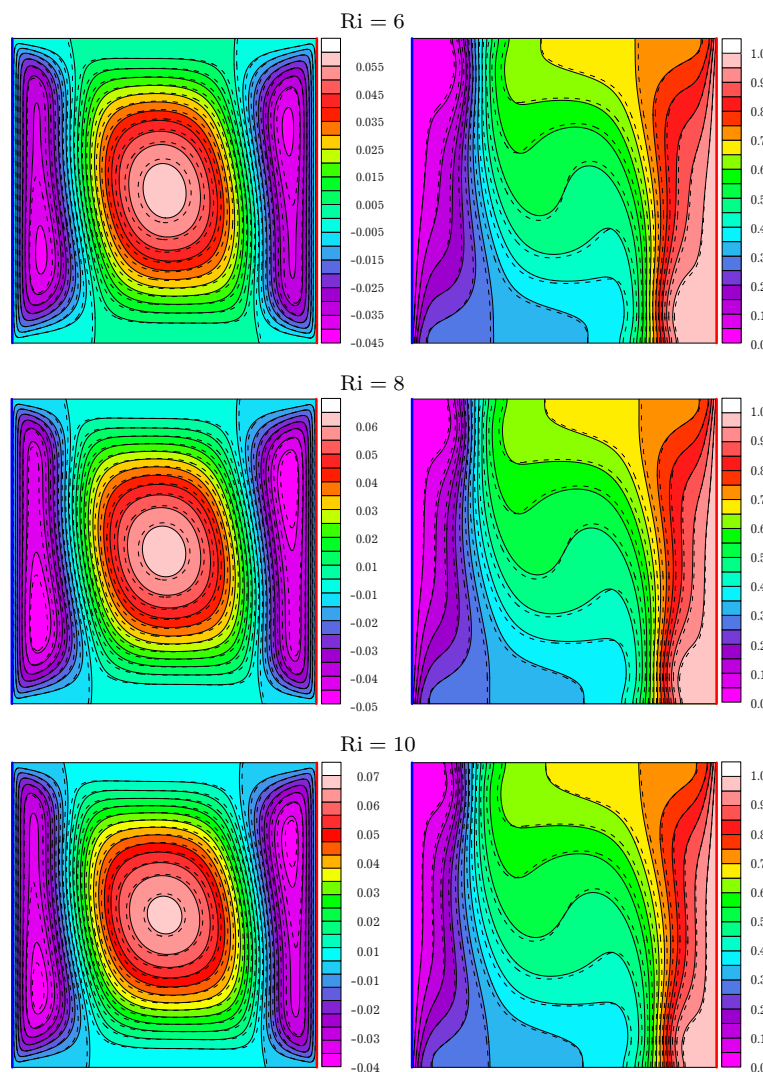
Fig. 3. Streamline shapes (left) and isotherm contours (right) of water (dashed line) and copper-water nanofluid (solid line) for various values of Ri , when \chi = 0.01 and d_{np} = 30 nm.
