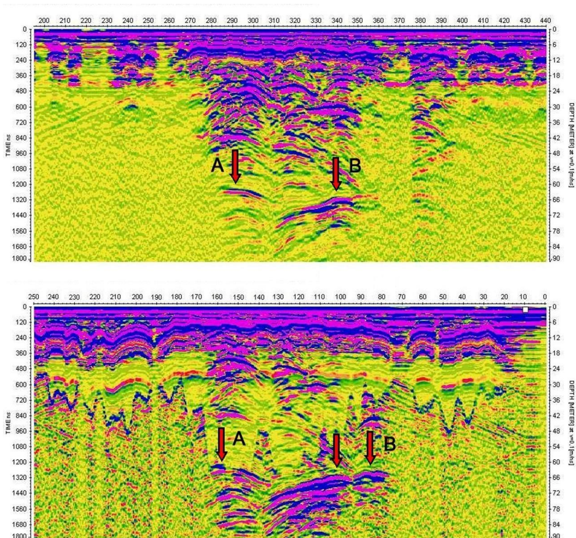
Fig. 9. Radarograms on profiles Sloup005 and Sloup006 above Amatérská cave (according to [Tengler et al., 2016])
