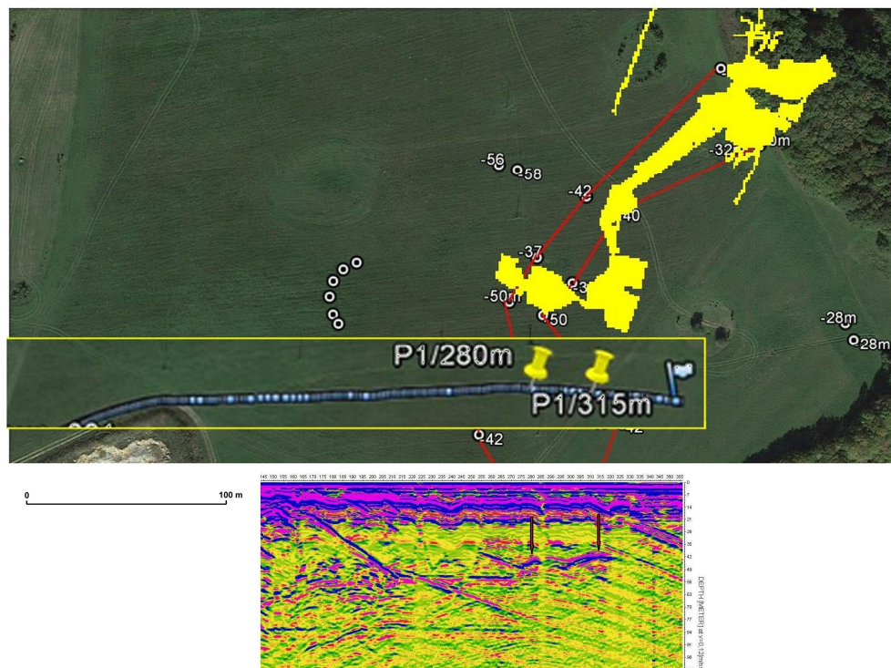
Fig. 7. Radarogram on profile P1 above Holštejnská cave (between distances 280 m and 315 m) (according to [Tengler et al. 2016])
