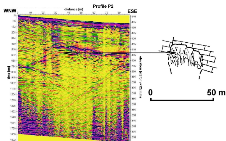
Fig. 13. Radarogram on profile P2 above Pretnerjeva Dvorana. Cross-section by [Gospodarič, 1985] (according to [Kalenda et al., 2018b])
