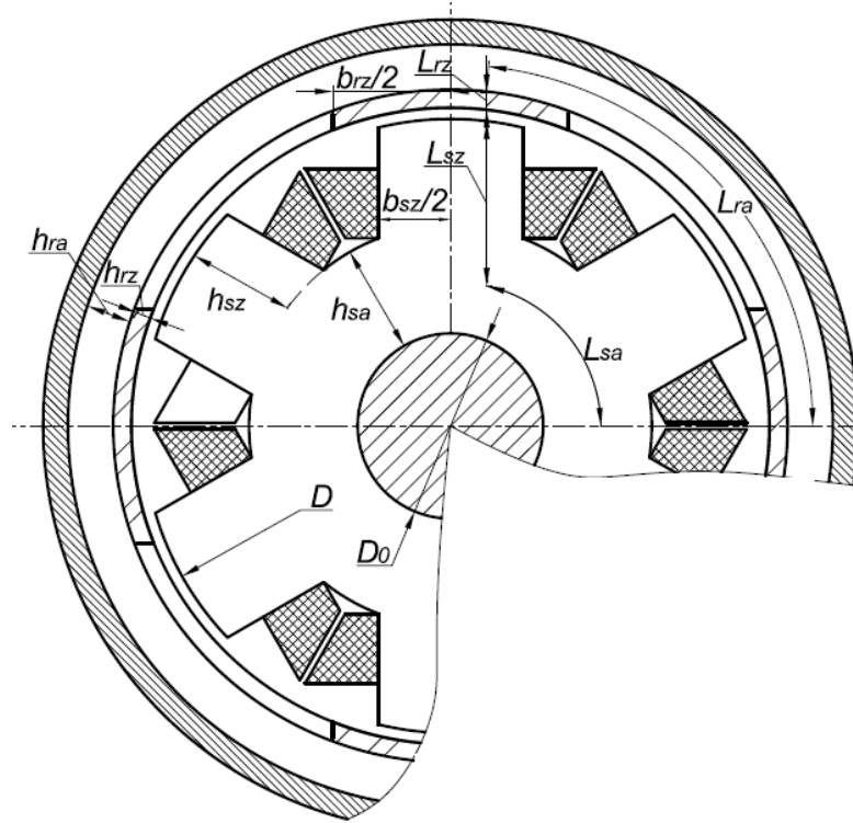
Fig. 1. Cross section of BLDC motor with external rotor
