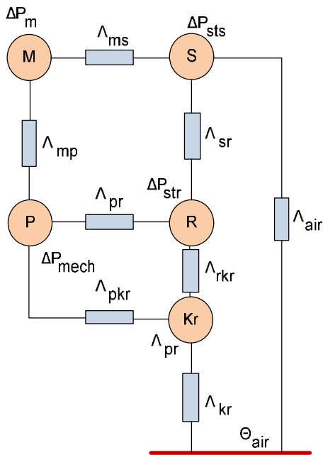
Fig. 2. Scheme for heat calculus of motor with external rotor [14]
