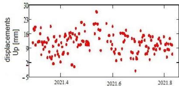
Fig. 9. Time series of the altitude component of the GNSS station
