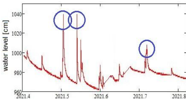
Fig. 11. Time series of changes in the groundwater level in the borehole
