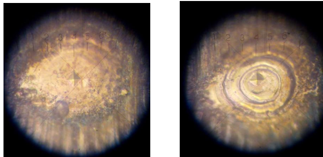
Fig. 3. Impressions of the indenter in the crater, which is formed by pulsed laser treatment of the aluminum surface
