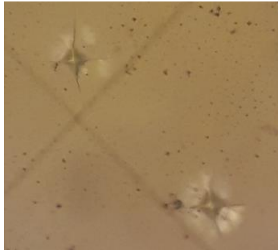
Fig. 6. Indenter prints on a clean SiC surface
