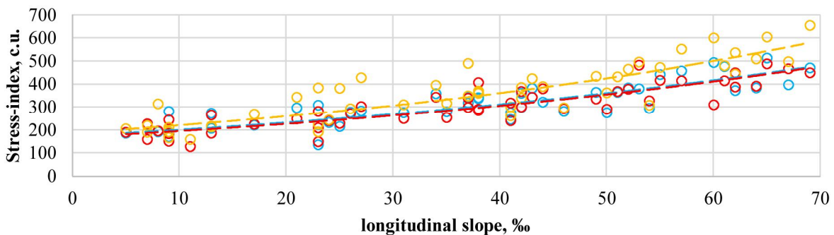
Fig. 5. Change of SI drivers, depending on the value of the longitudinal slope at a load level Z > 0.5 when transporting dangerous goods by road, for the studied groups: --- Group 1 --- Group 2 --- Group 3
