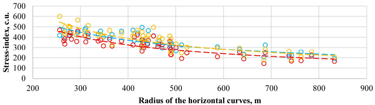
Fig. 4. Change of driver's SI, depending on the radius of horizontal curves at the load level Z > 0.5 when transporting dangerous goods by road, for the studied groups: --- Group 1 --- Group 2 --- Group 3
