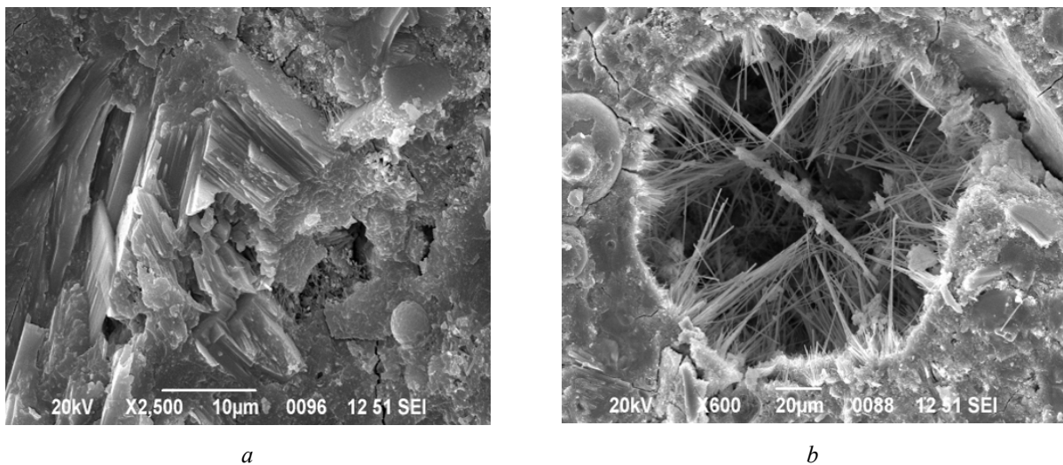
Fig. 5. Microstructure of paste based on superplasticized cementitious systems after 28 days of hardening
