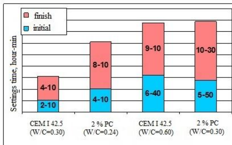
Fig. 2. Setting time of cement systems with polycarboxylate superplasticizer
