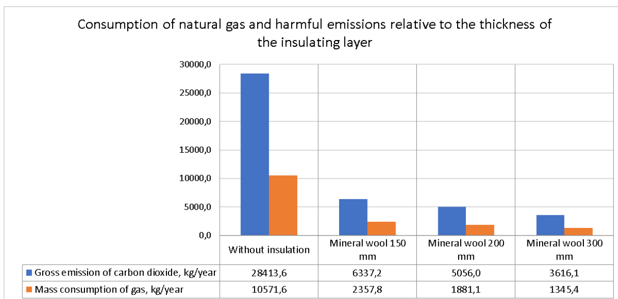
Fig. 5. Natural gas consumption for heating the school building and carbon dioxide emissions with insulation thicknesses of 150 mm, 200 mm and 300 mm
