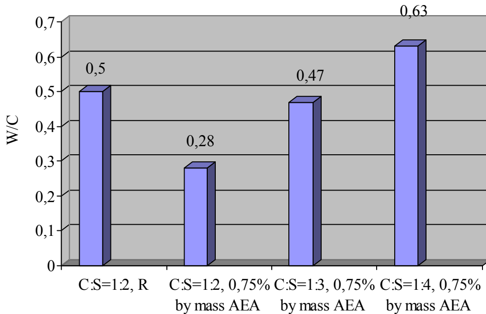
Fig. 2. W/C ratio of mortars with the different proportions of cement to sand ( F=125-135 mm)
