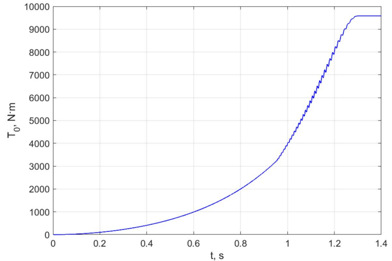
Fig. 5. Dependence of the turning resistance moment of the steered wheels on time
