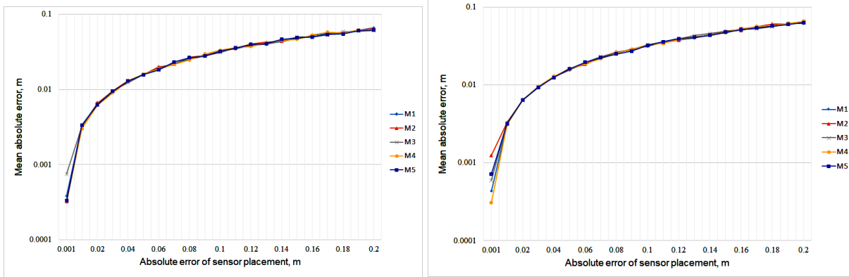
Fig. 7. Dependence of MAE on the absolute sensor detection error: a) X coordinate, b) Y coordinate
