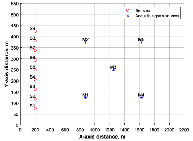
Fig. 2. Location of sensors and sound sources
