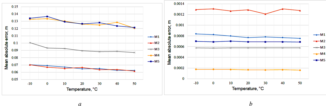
Fig. 8. MAE values with correction factor: a) X coordinate, b) Y coordinate
