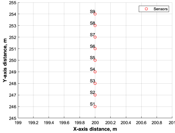
Fig. 5. Sensor placement with a distance of 1 m between them
