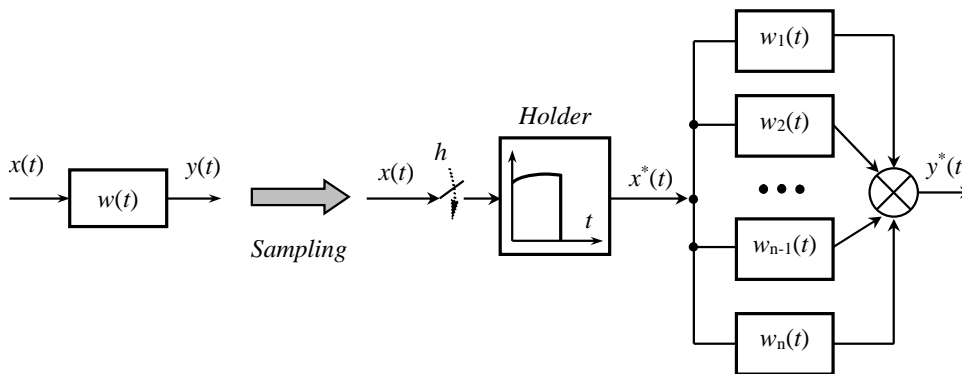
Fig. 3. Parallel decomposition of the continuous transfer function
