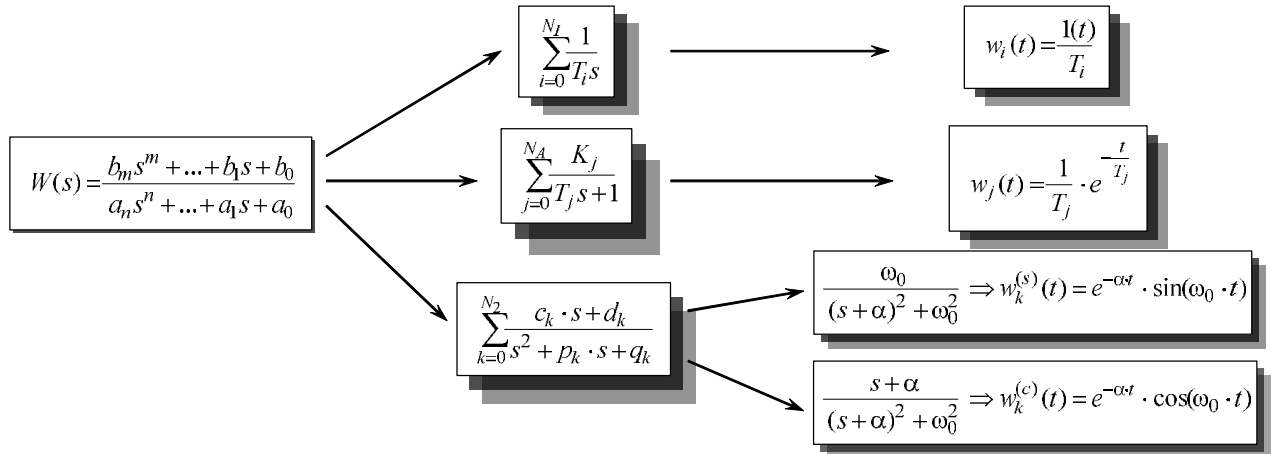
Fig. 1. Decomposition scheme of the transfer function into elementary components
