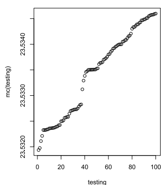
Fig. 3. Prediction by \hat{m}_V (right panel), \hat{m}_R (middle panel) and \hat{m}_C (left panel).
