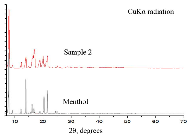
Fig. 10. Comparison of diffractograms of menthol from 25 and sample 2
