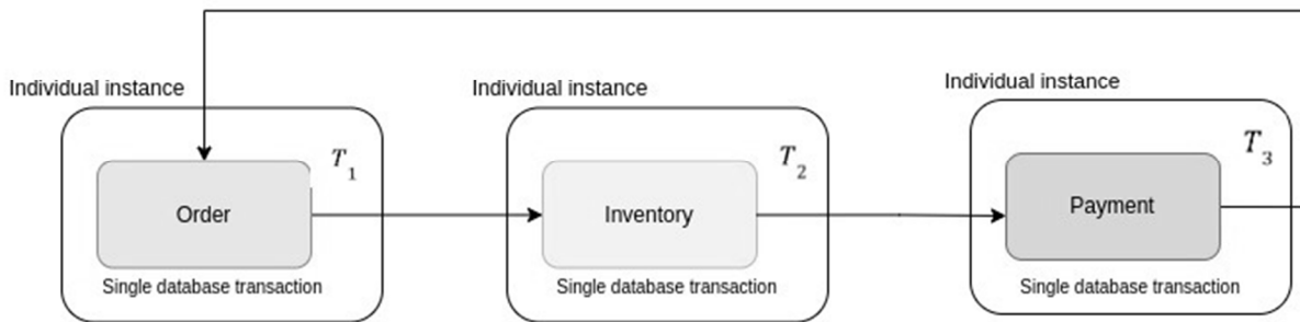
Fig. 2. Microservices architecture( )
