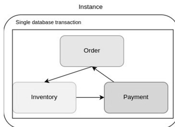
Fig. 1. Monolith architecture ( )
