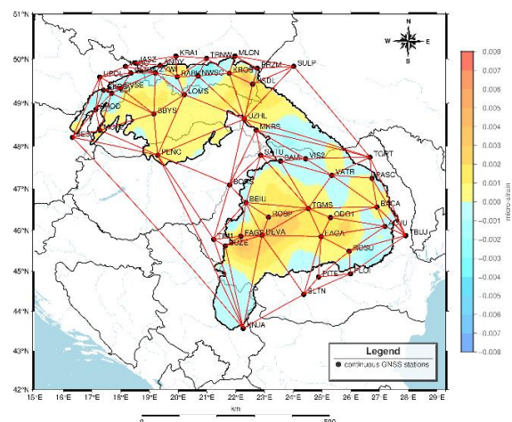
Fig. 8. Distribution of dilatation rates velocities.
