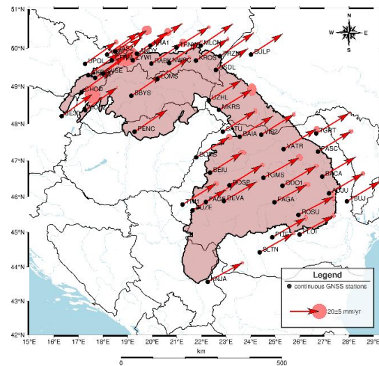
Fig. 5. Distribution of absolute velocity vectors of horizontal movements.
