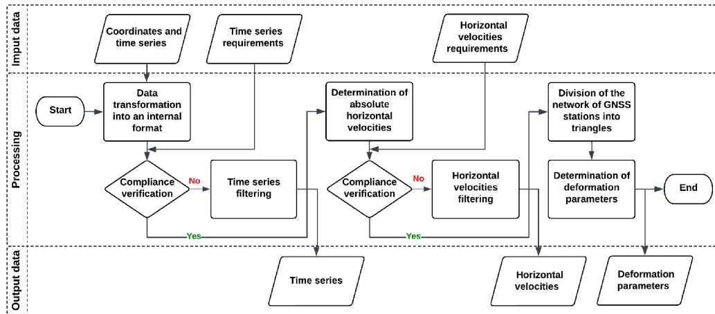
Fig. 3. Algorithm for determining deformation parameters based on GNSS measurement data.
