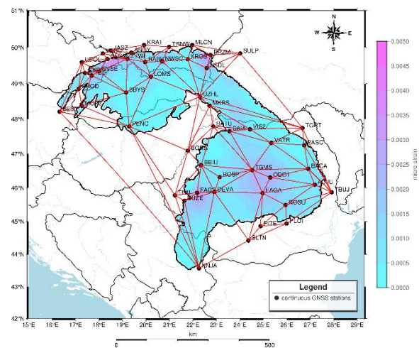
Fig. 7. Distribution of total shear rates velocities.
