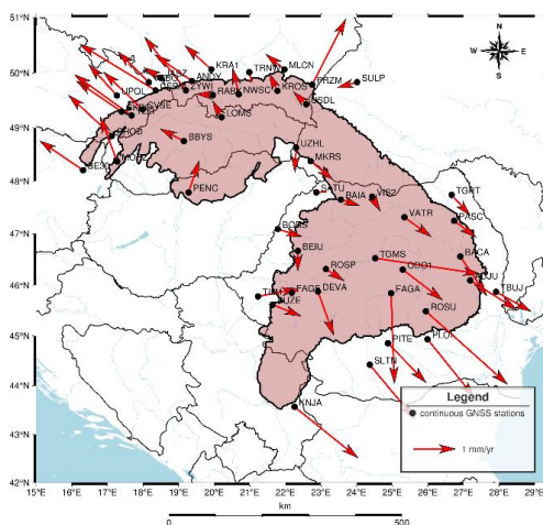
Fig. 6. Distribution of regional velocities vectors of horizontal movements.
