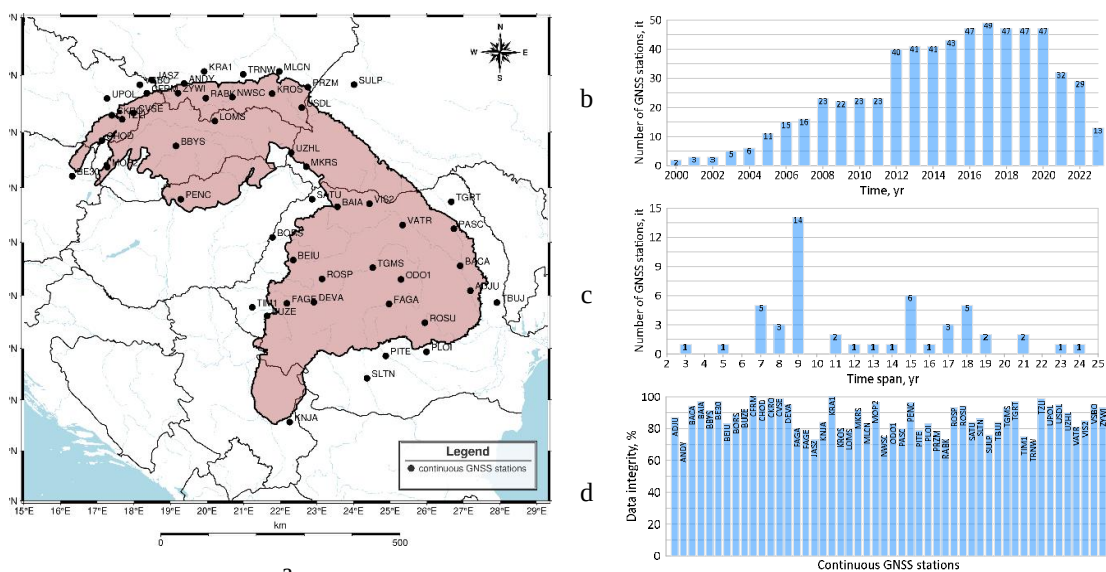
Fig. 2. Continuous GNSS station network of Carpathian Mountain and characteristics (a) of station availability (b), station time span (c) and station data integrity (d).
