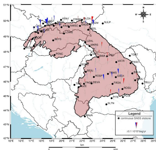
Fig. 9. Distribution of rotation rates velocities.
