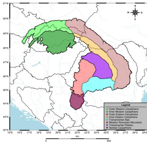
Fig. 1. The diagram of the Carpathian mountain system.
