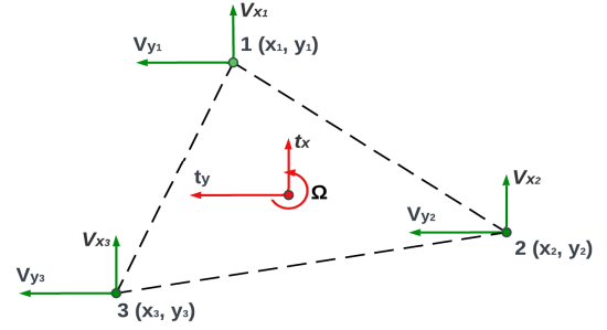
Fig. 4. Scheme of deformations within one triangle.
