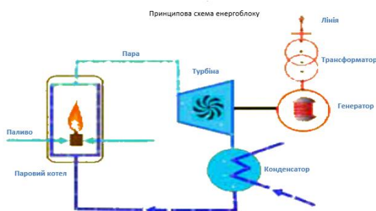
Fig. 6 Schematic diagram of the power unit.
