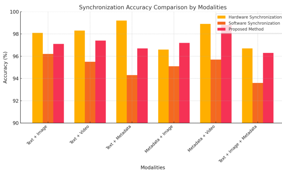
Fig. 3. Comparison of synchronization method approaches
