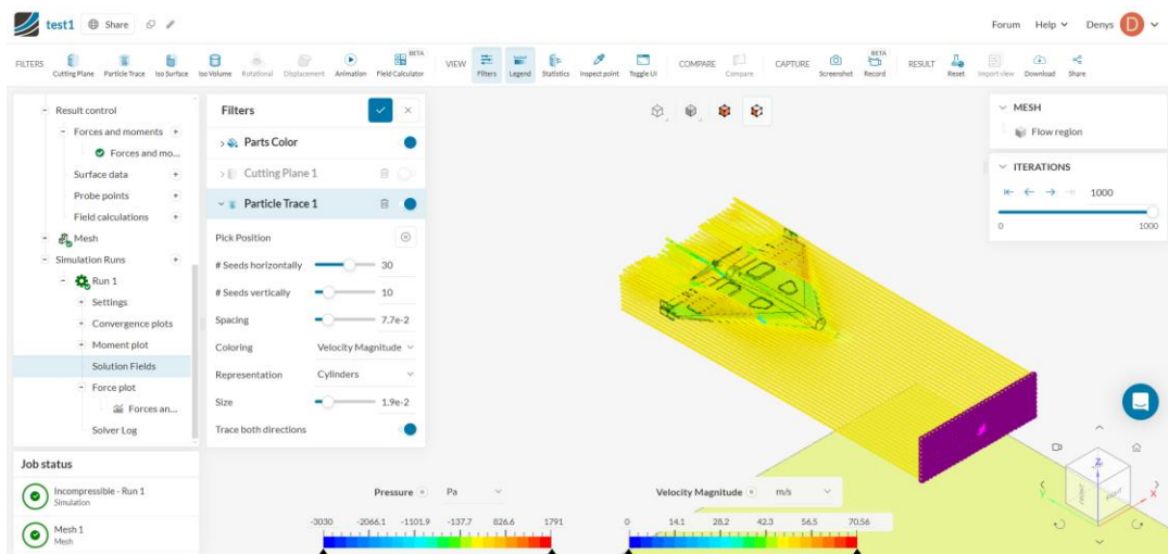
Fig. 13. Visualisation of air flow during the simulation.
