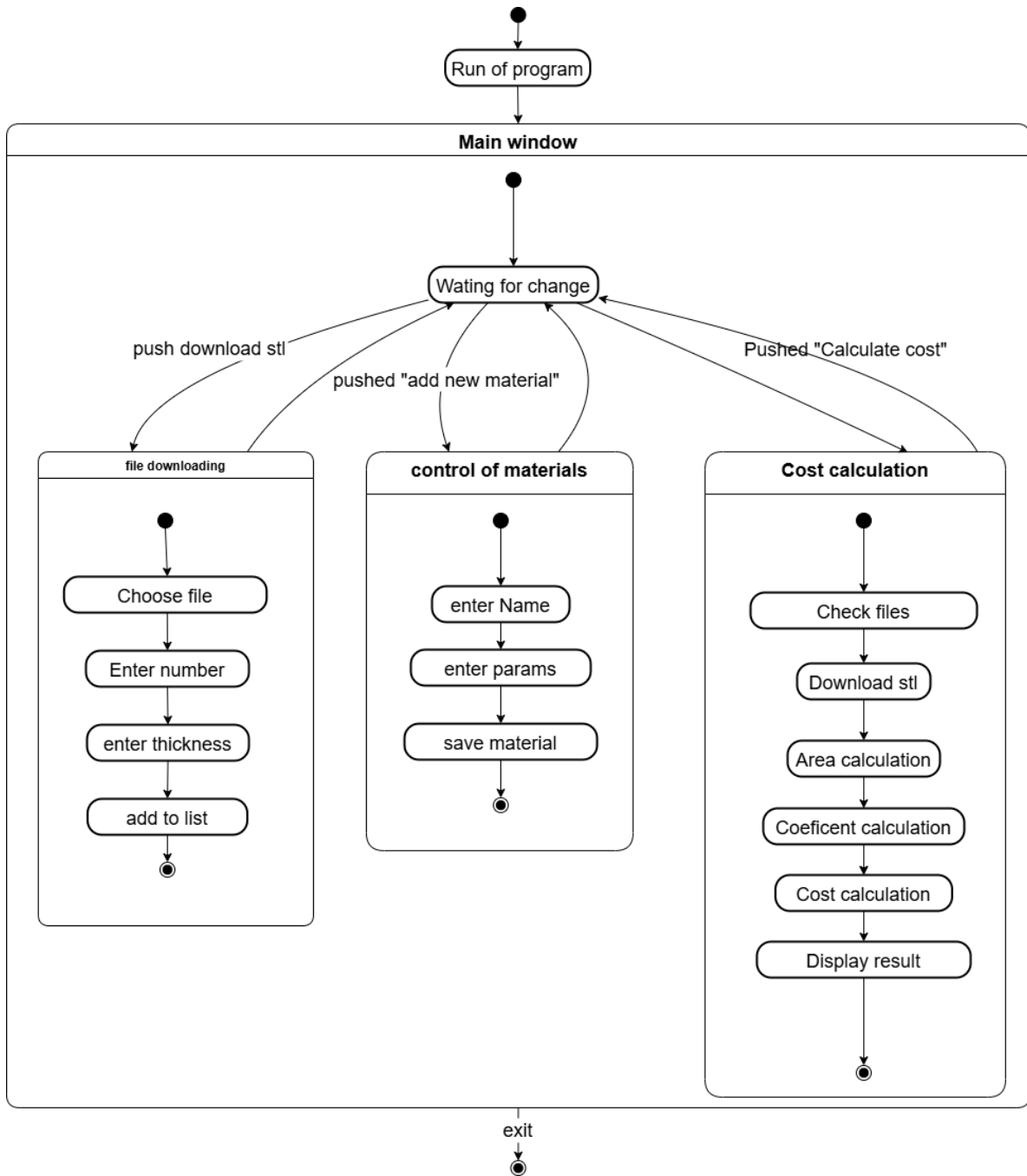
Fig. 15. Activity diagram
