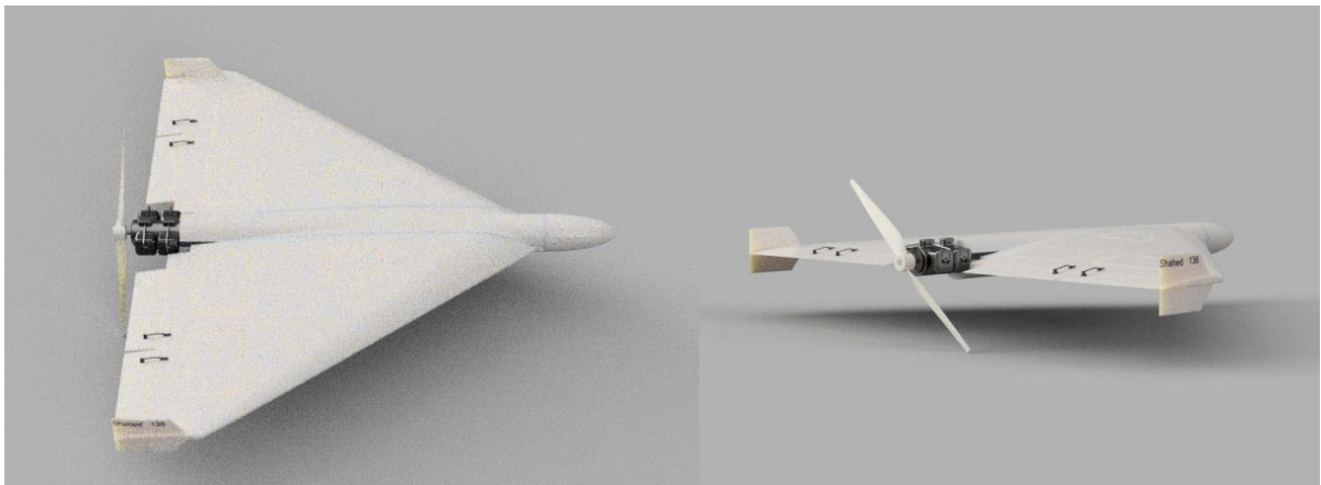
Fig. 12: Rendering result
