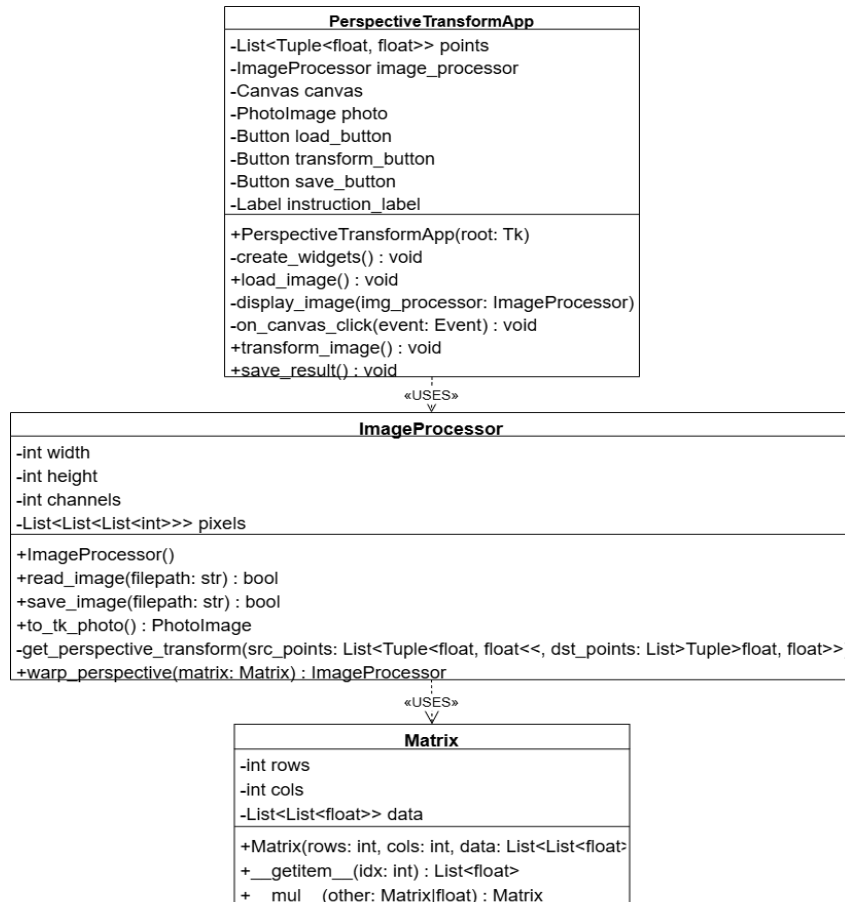
Fig. 3. Class diagram of the software solution
