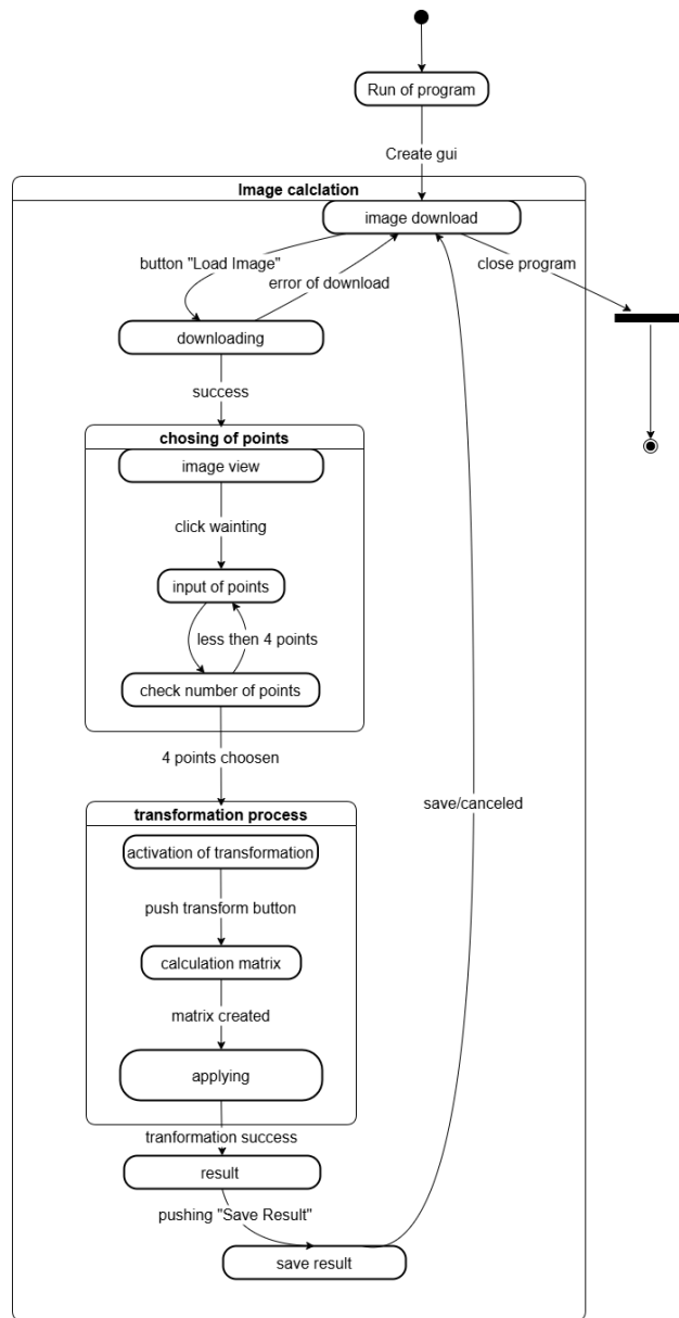
Fig. 5. Diagram of activities during image transformation
