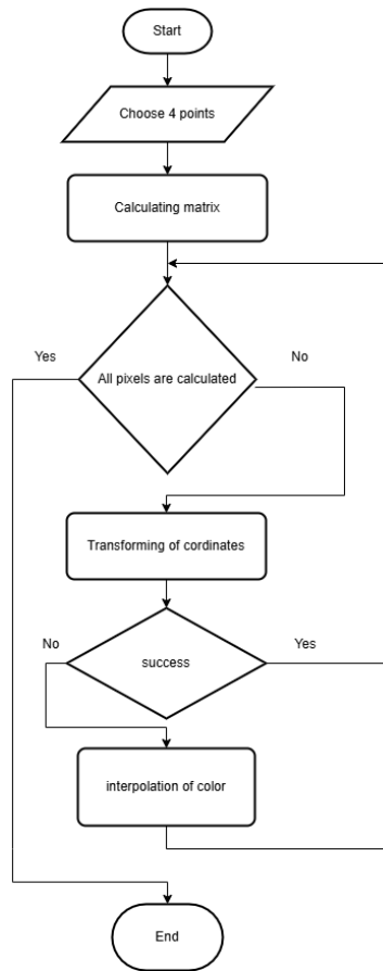
Fig. 2. Image transformation flowchart
