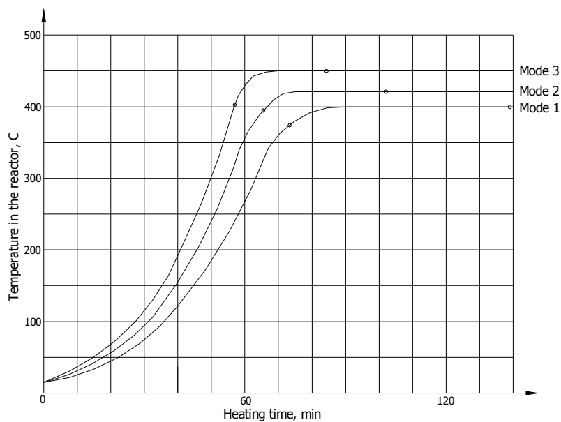
Fig. 1. Polyethylene waste pyrolysis modes
