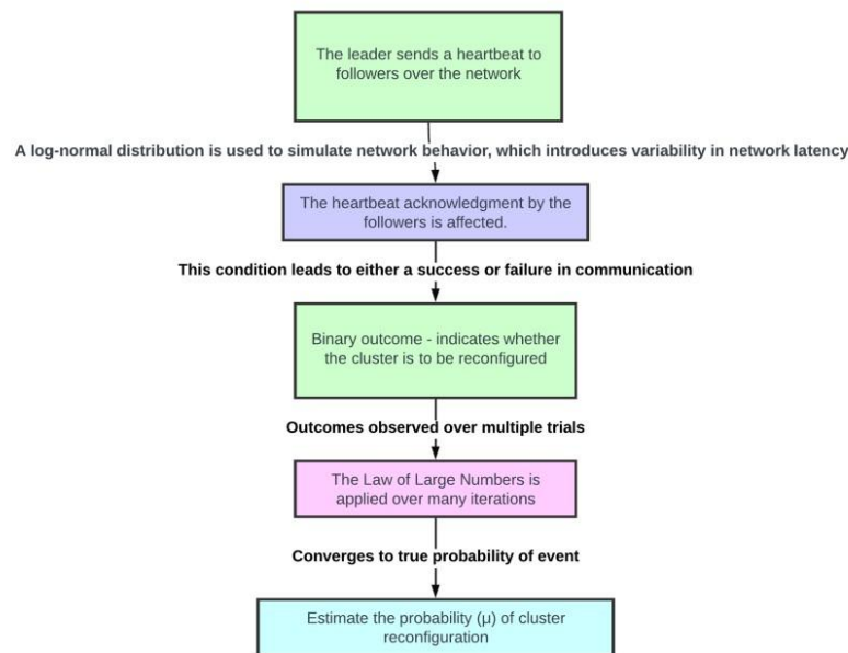
Fig. 8. Flowchart for estimating the probability of cluster reconfiguration due to network latency
