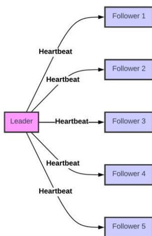
Fig. 7. Leader-node heartbeat communication diagram
