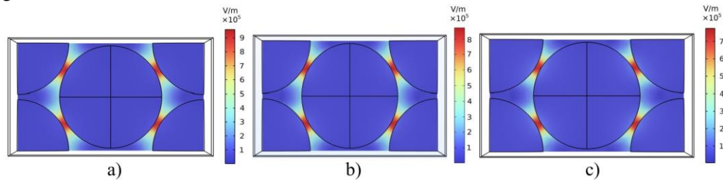
Fig.4. Distribution of the electric field of a normally incident electromagnetic wave with Au nanoparticles array with a radius of 10 nm and a gap between the nanoparticles surfaces of 1 nm in the surrounding media with refractive index of 1.00 (a), 1.33 (b) and 1.43 (c). The colour bar indicates the electric field intensity under the wavelength of 650 nm.
