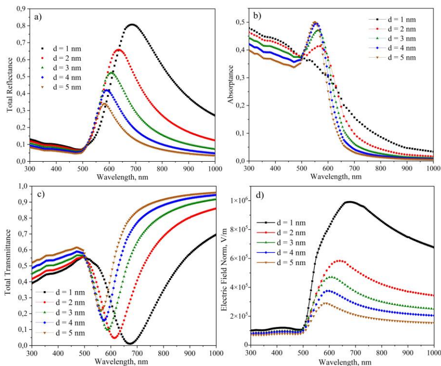
Fig.3. The total Reflectance (a), Absorbance (b), Transmittance (c) and Electric field distribution (d) spectra of Au nanoparticles array with a radius of 10 nm and a gap between the surface of the particles from 1 to 5 nm in a surrounding media with a refractive index of 1.33
