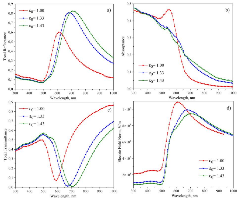
Fig.5. The total Reflectance (a), Absorbance (b), Transmittance (c) and Electric field distribution (d) spectra of Au nanoparticles array with a radius of 10 nm and gap between the nanoparticles surfaces of 1 nm in the surrounding media with variable refractive index.
