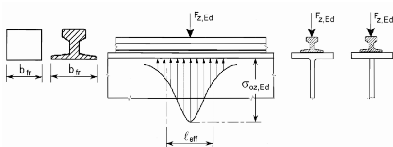
Fig. 4. Effective load length according to EN 1993-6 (2007)
