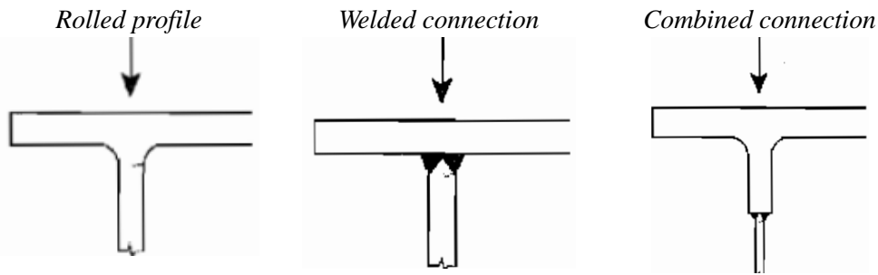
Fig. 2. Different types of web-flange connections in runway beams
