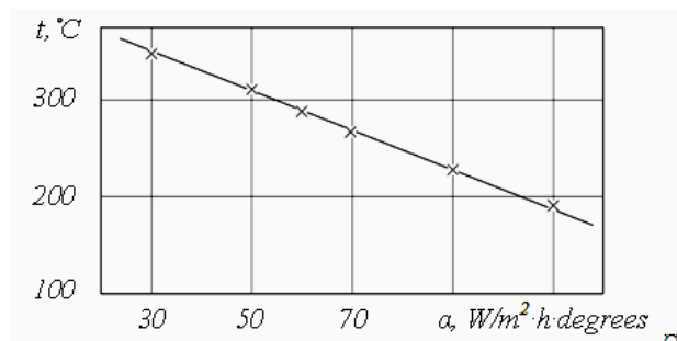
Fig. 3. The influence of \alpha on the temperature of the brake drum at the end of the preliminary stage of test I
