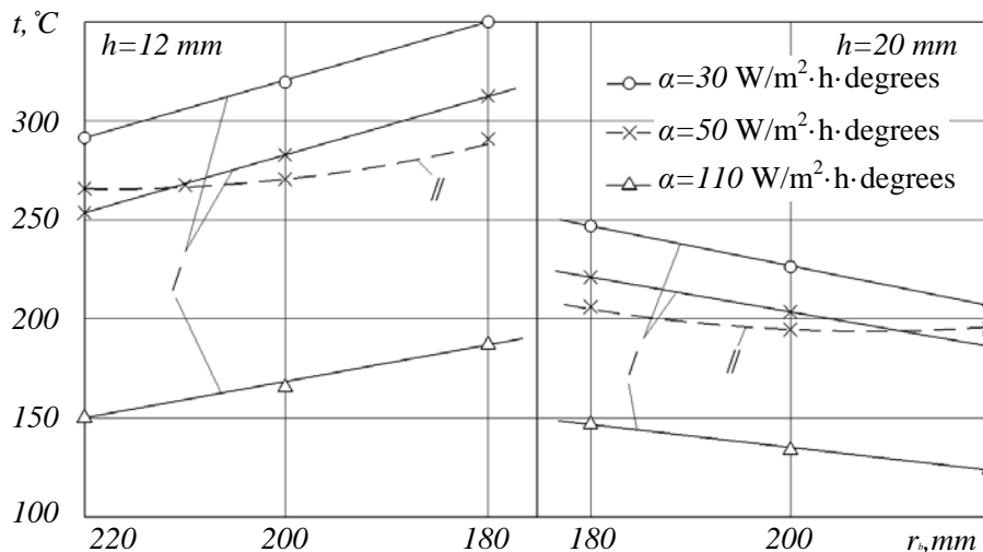
Fig. 2. Dependence of brake drums temperature at the end of the preliminary stage of test I from r_b ( b=80 mm): I – without considering changes in \alpha ; II – considering \alpha=f(S)
